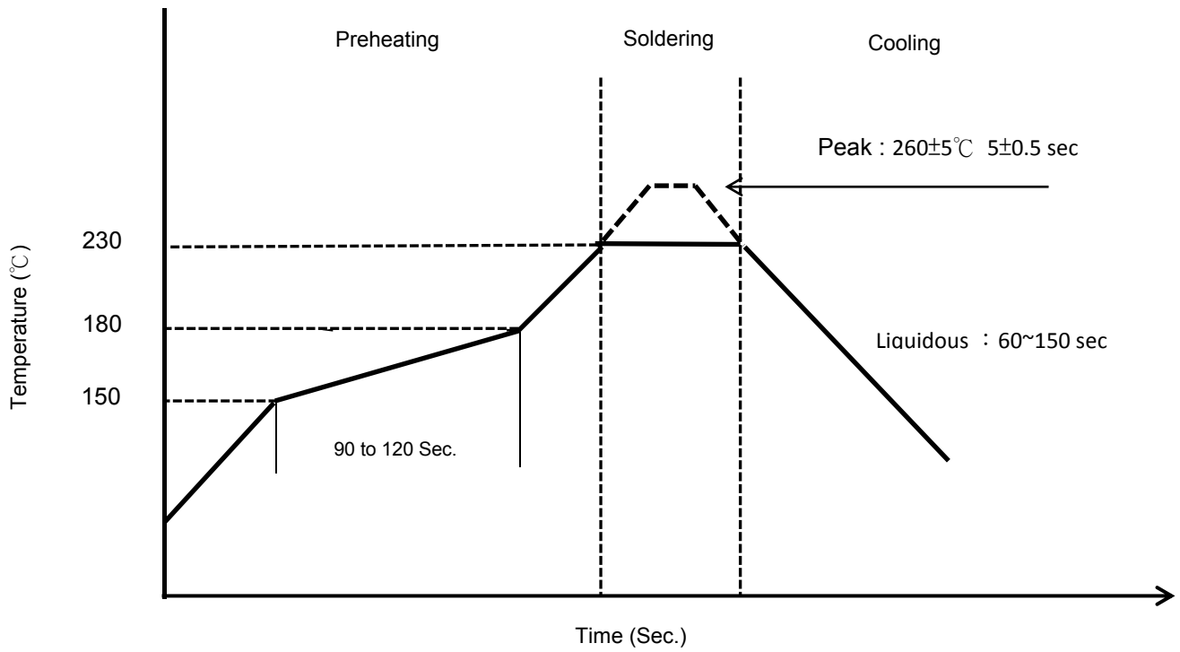
Figure 1. Re-flow Soldering
