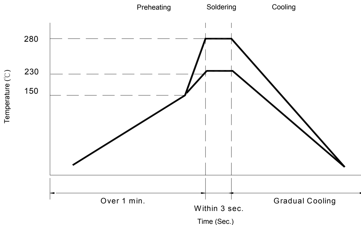
Figure 2. Hand Soldering
