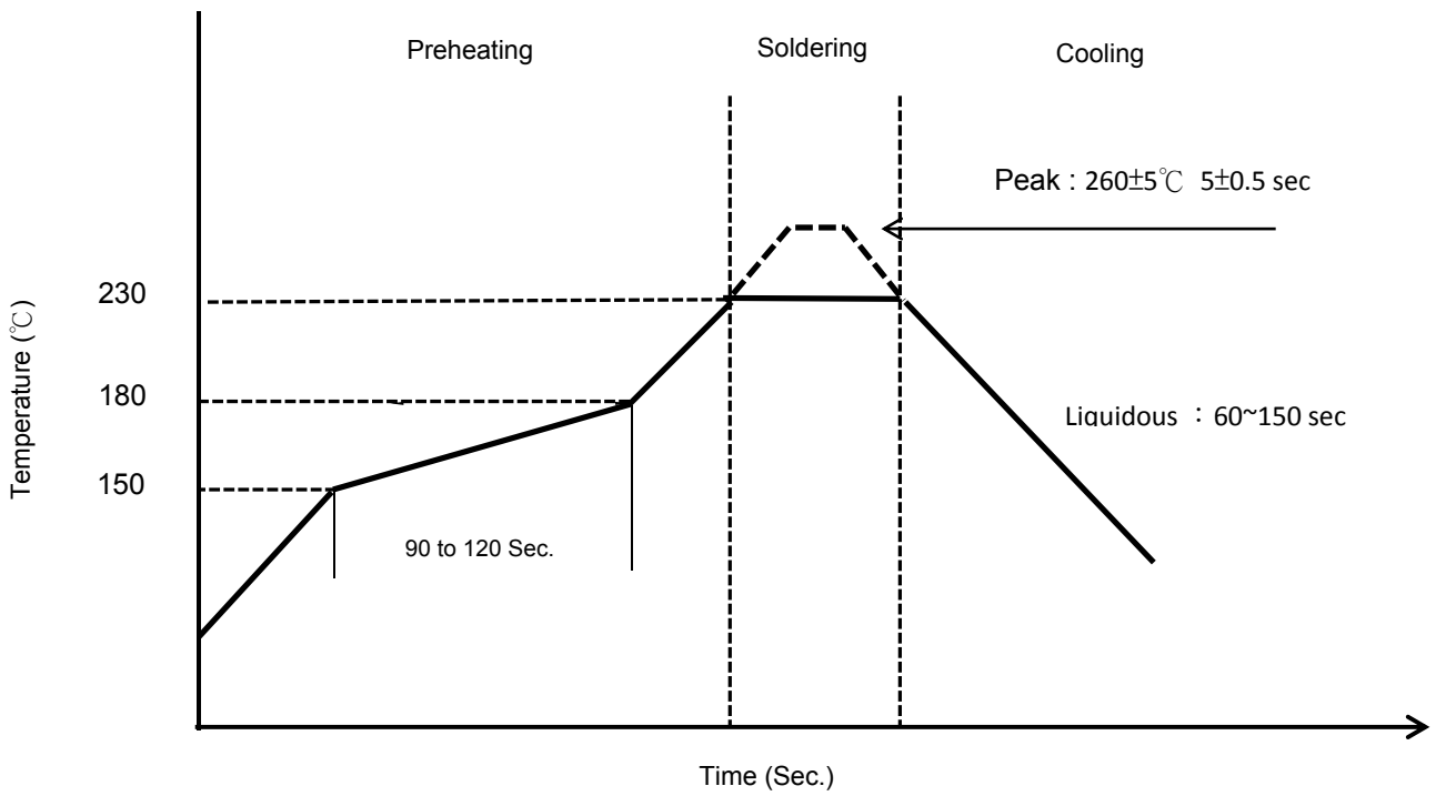
Figure 1. Re-flow Soldering
