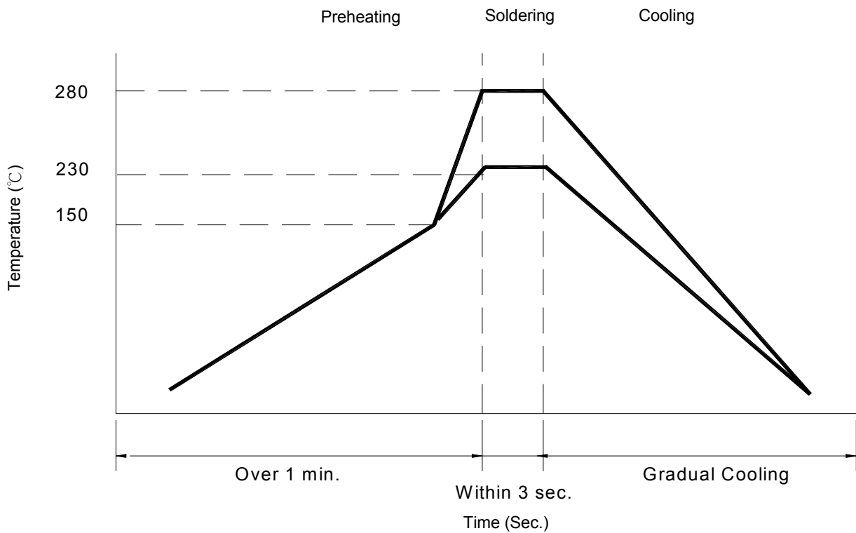
Figure 2. Hand Soldering
